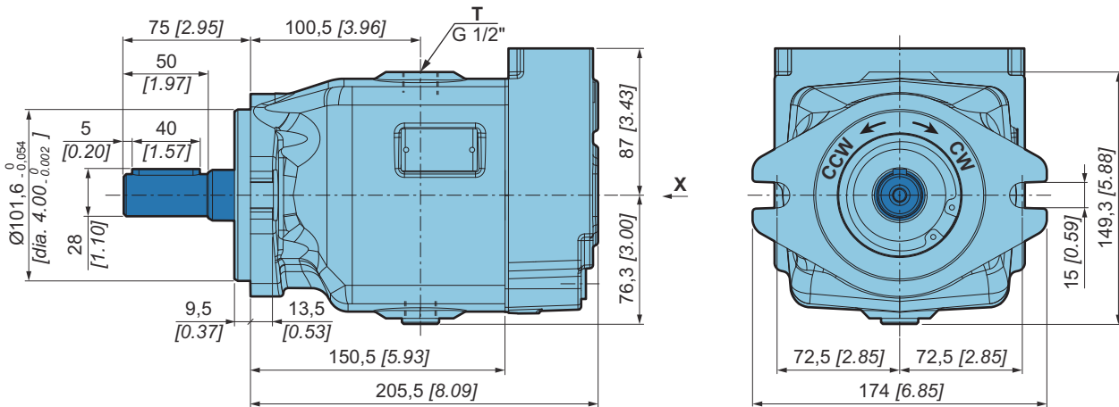
VIEW "X"
