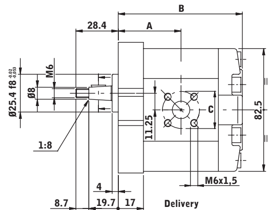
Delivery
