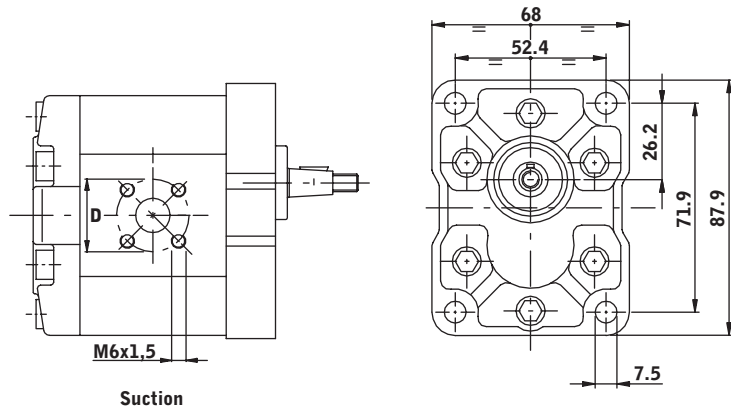
Suction
